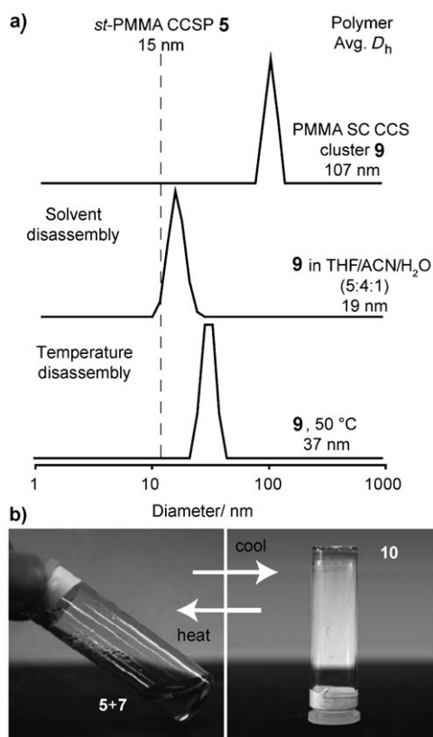
Figure 4. a) Disassembly of the PMMA SC 9 can be induced by the addition of a good solvent (e.g. THF) or by heating. b) Similarly, the PMMA SC gel 10 can be switched between solution and solid states by heating/cooling.
